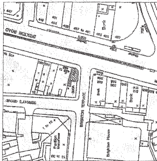
D.S. SITE LOCATION PLAN - Scale 1 : 1250
